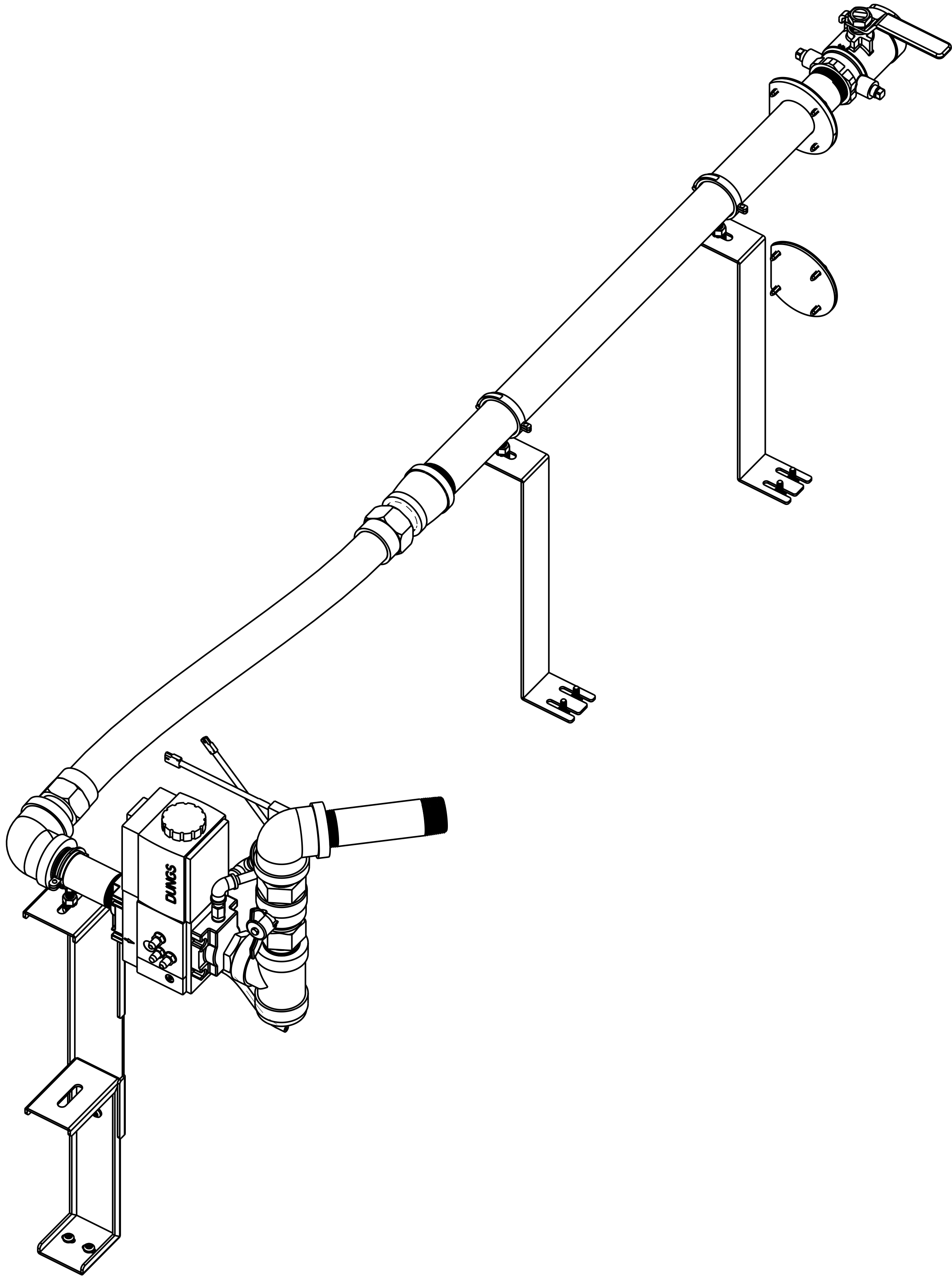
ISOMETRIC SCALE 0.313
