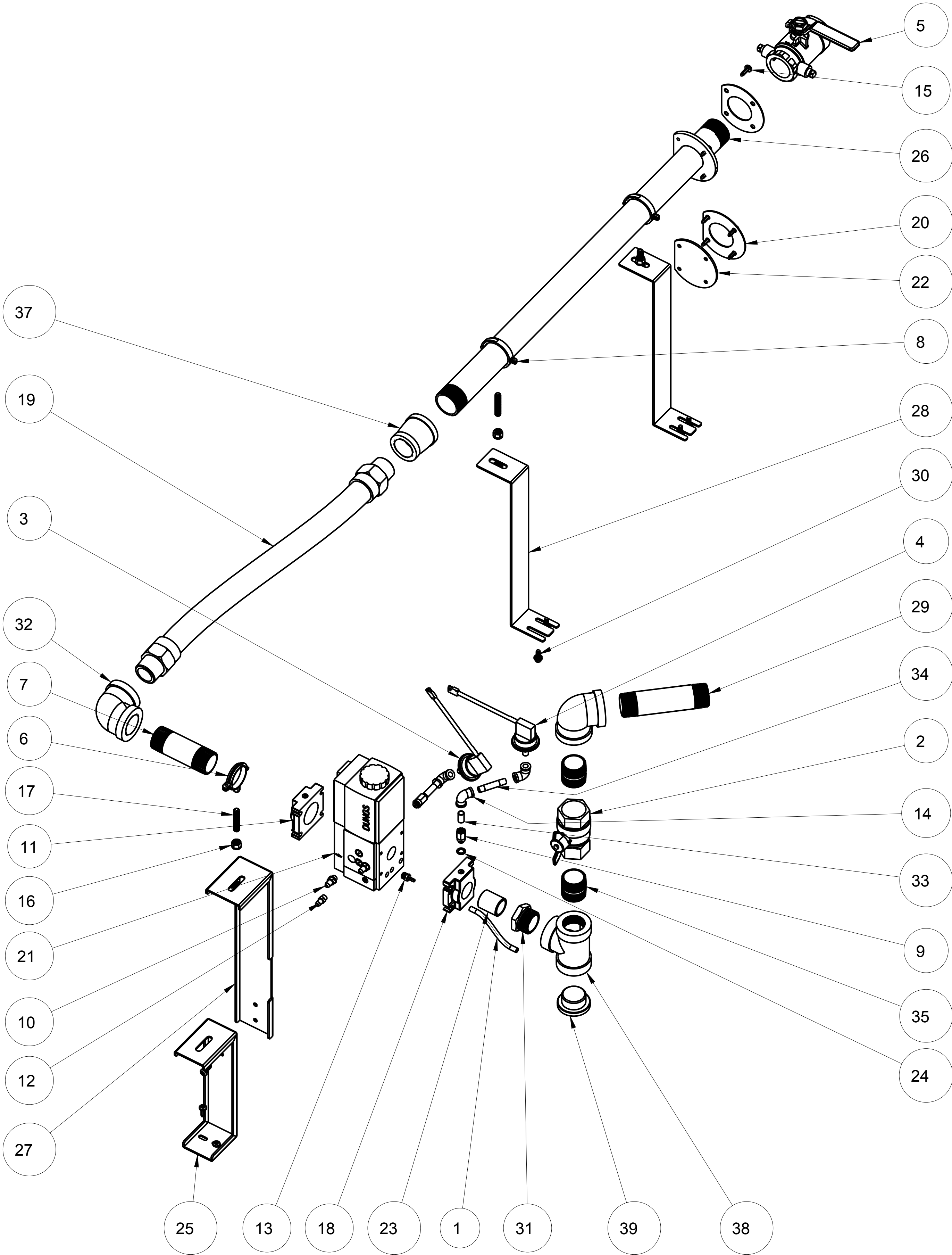
EXPLODED SCALE 0.219
