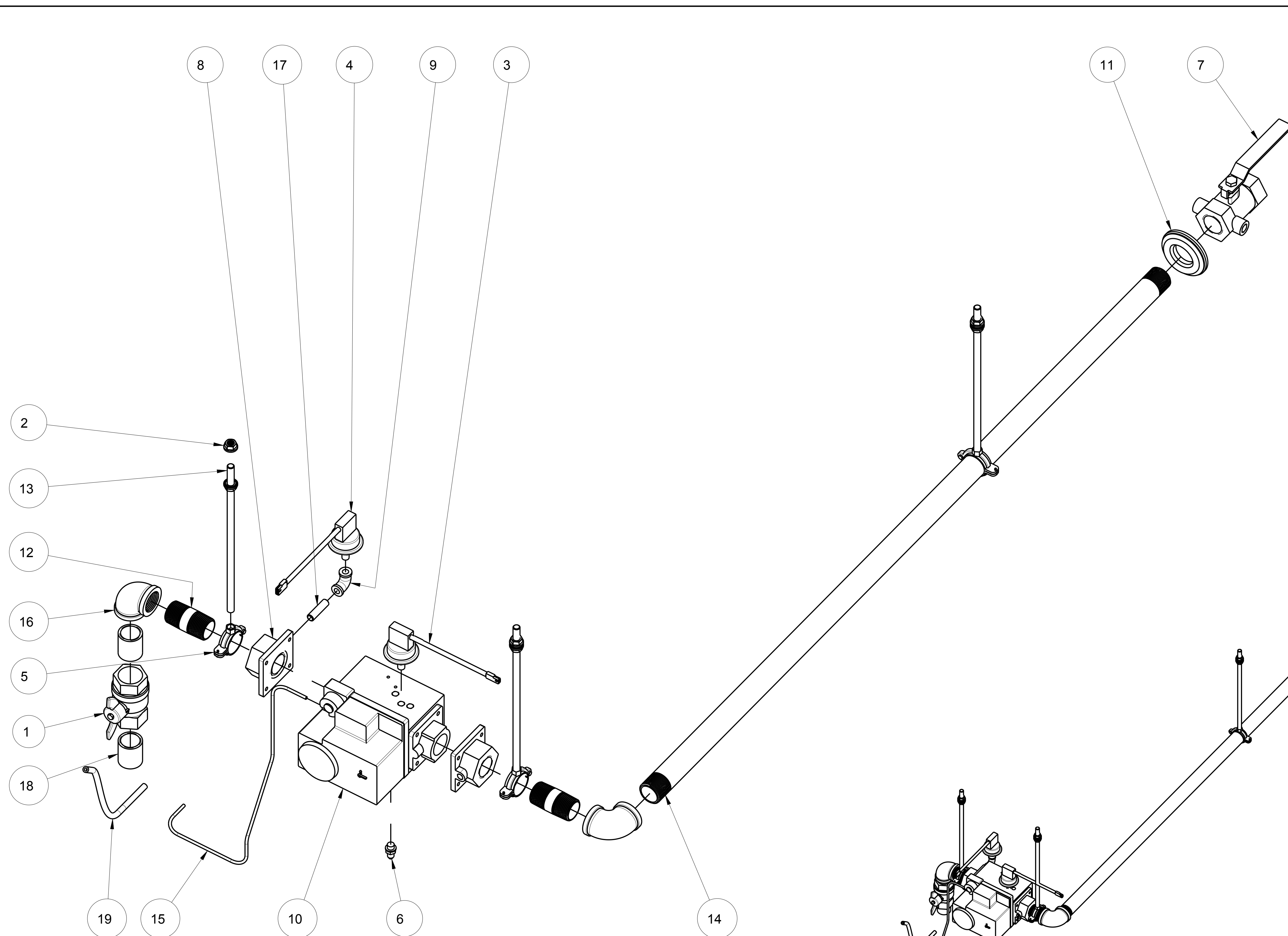
EXPLODED SCALE 0.344
