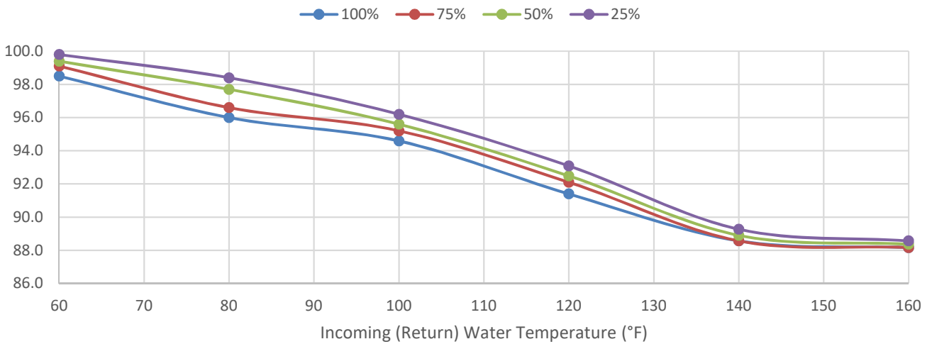
SONIC SC-2000 Thermal Efficiencies @ 40°F ΔT
