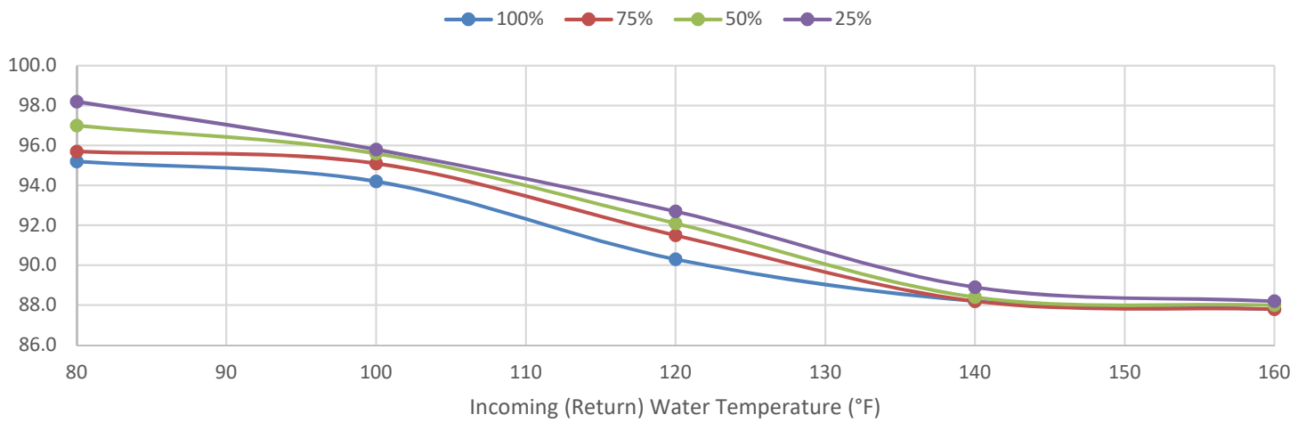
SONIC SC-4000 Thermal Efficiencies @ 60°F ΔT
