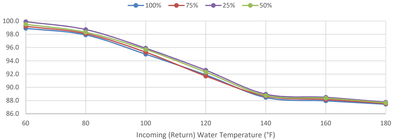
SONIC SC-2000 Thermal Efficiencies @ 20°F ΔT
