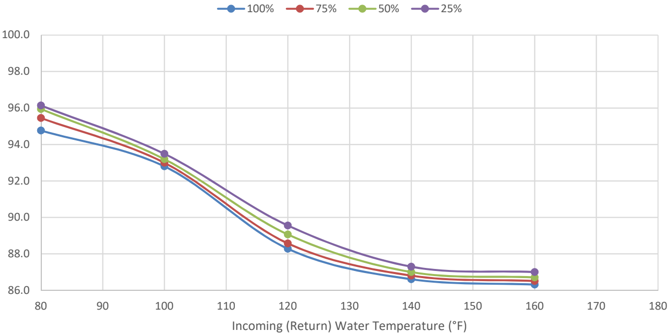
SONIC SC-1000 Thermal Efficiencies @ 40°F ΔT
