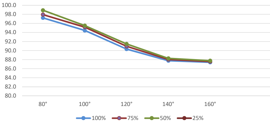
SONIC SC-650 Thermal Efficiencies @ 20°F ΔT
