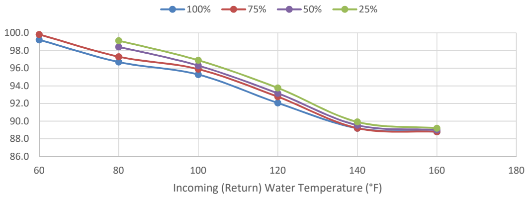
SONIC SC-1500 Thermal Efficiencies @ 40°F ΔT
