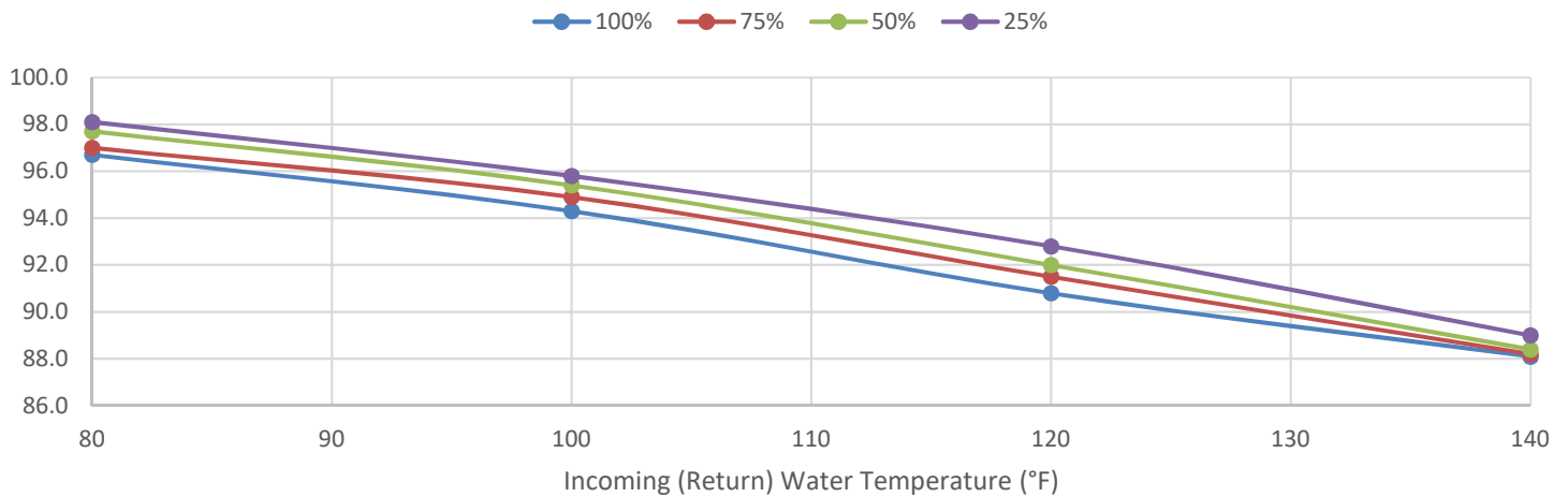
SONIC SC-4000 Thermal Efficiencies @ 60°F ΔT
