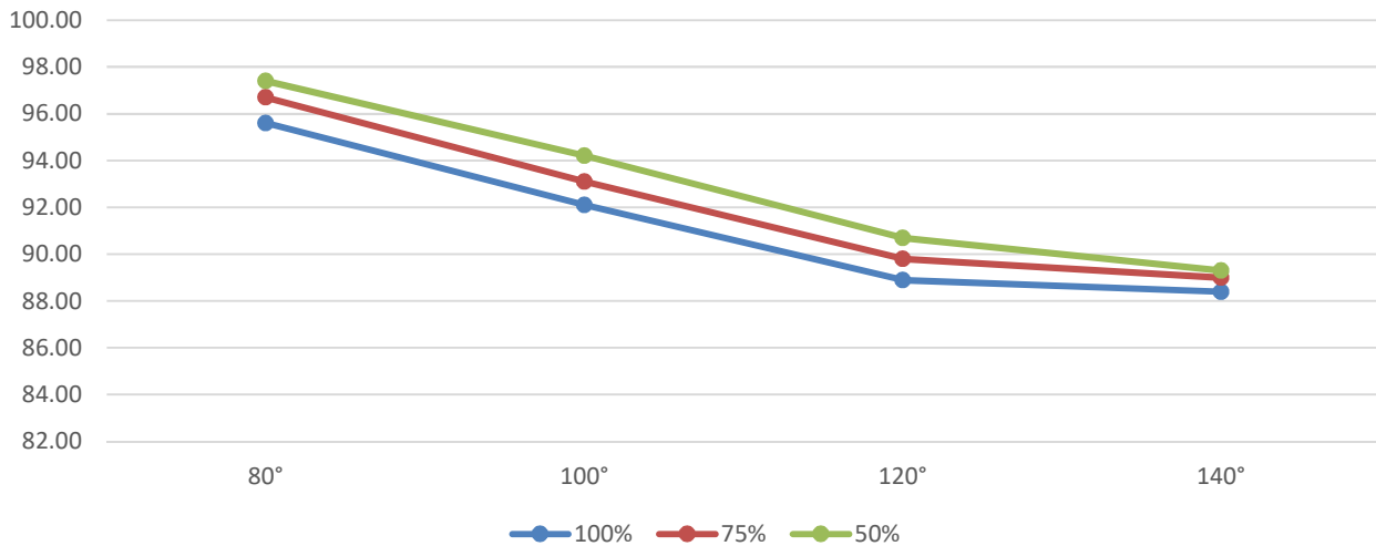
SONIC SC-750 Thermal Efficiencies @ 60°F ΔT
