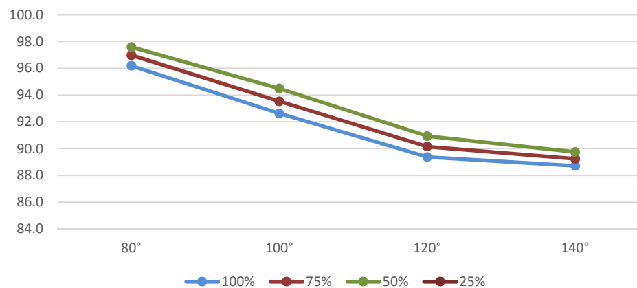
SONIC SC-650 Thermal Efficiencies @ 60°F ΔT
