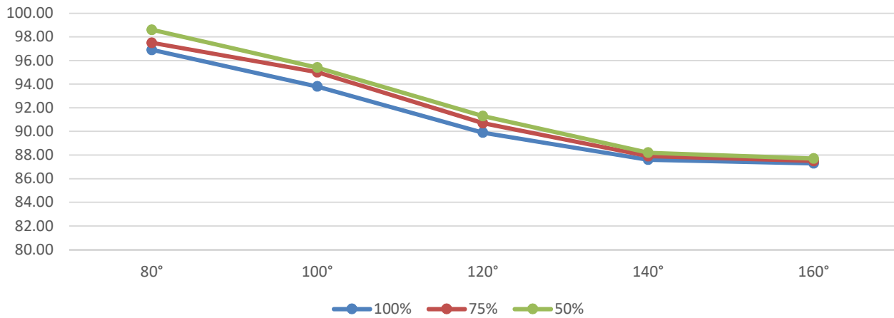
SONIC SC-750 Thermal Efficiencies @ 20°F ΔT
