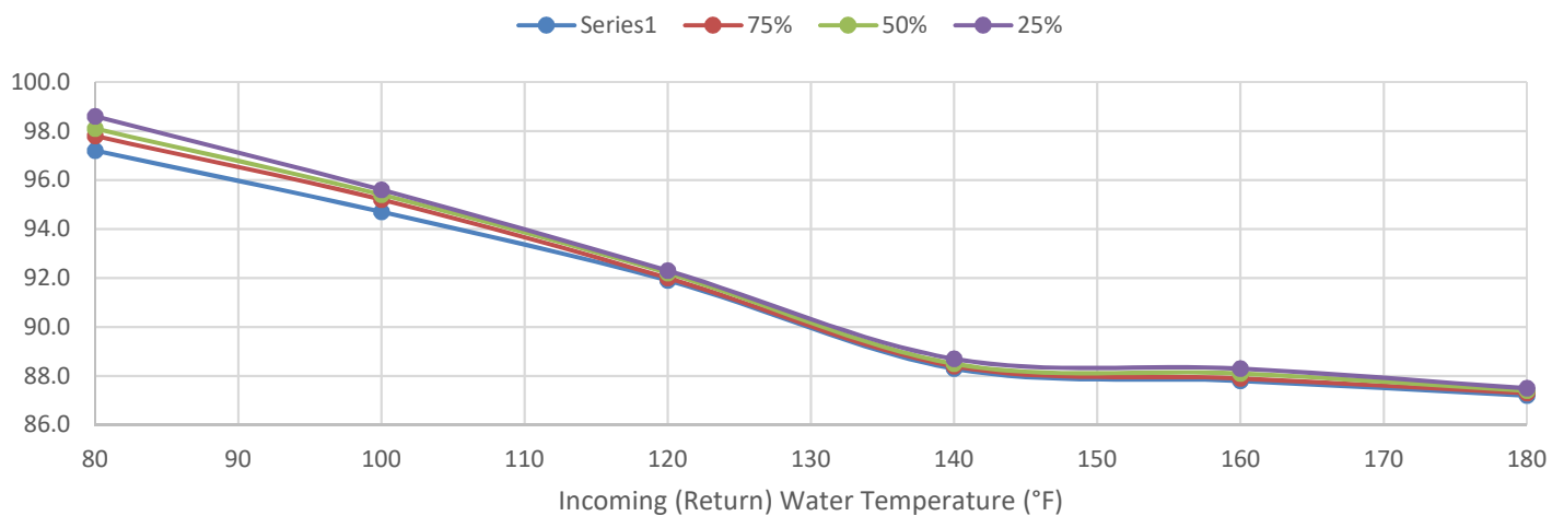
SONIC SC-3000 Thermal Efficiencies @ 20°F ΔT
