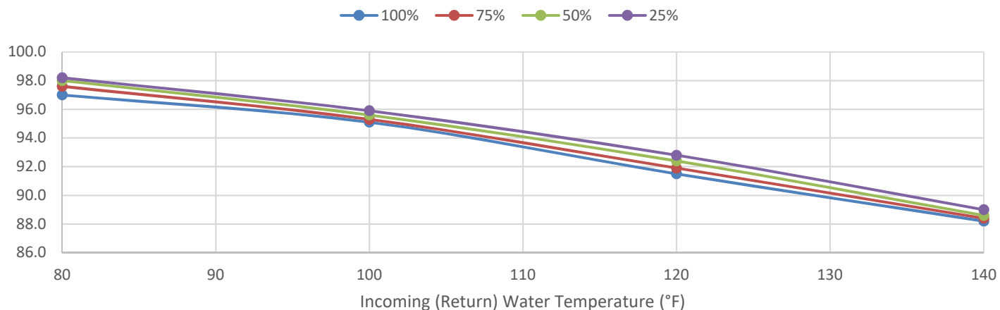
SONIC SC-3000 Thermal Efficiencies @ 60°F ΔT
