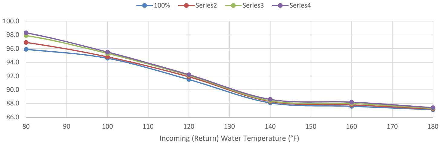
SONIC SC-4000 Thermal Efficiencies @ 20°F ΔT
