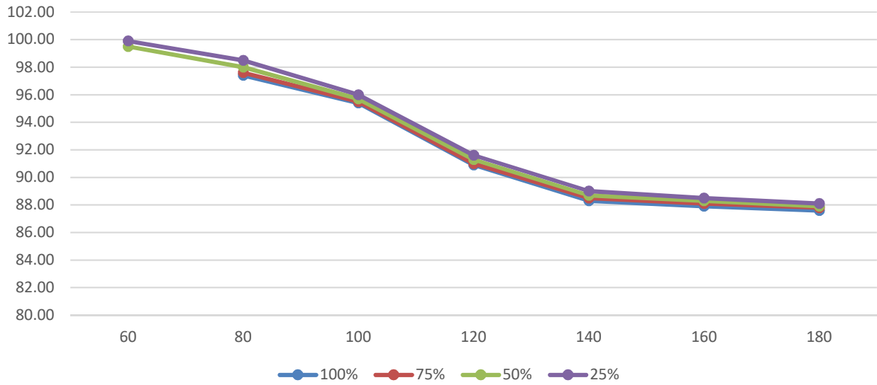
SONIC SC-850 Thermal Efficiencies @ 20°F ΔT
