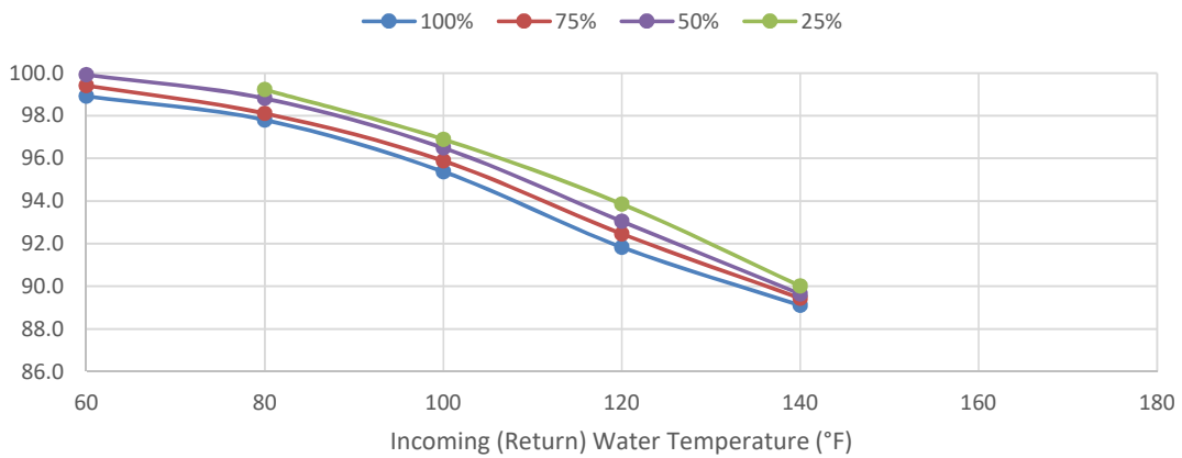
SONIC SC-1500 Thermal Efficiencies @ 60°F ΔT
