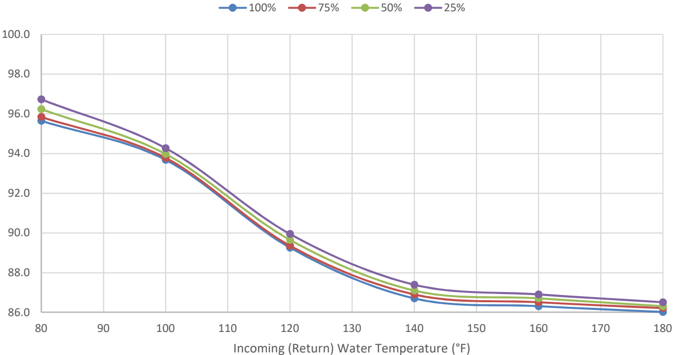
SONIC SC-1000 Thermal Efficiencies @ 40°F ΔT
