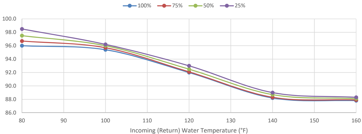
SONIC SC-3000 Thermal Efficiencies @ 60°F ΔT
