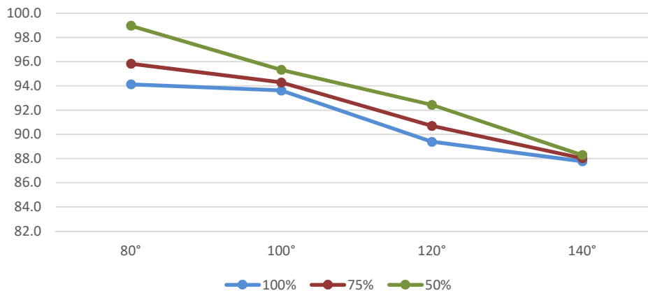
SONIC SC-650 Thermal Efficiencies @ 40°F ΔT
