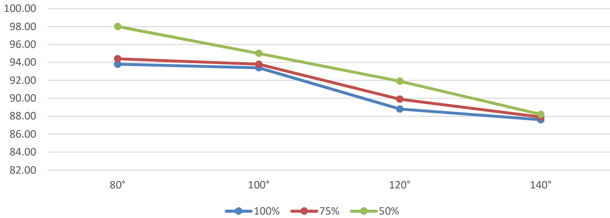
SONIC SC-750 Thermal Efficiencies @ 40°F ΔT
