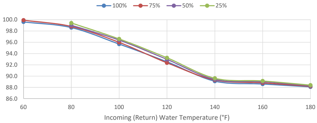
SONIC SC-1500 Thermal Efficiencies @ 20°F ΔT
