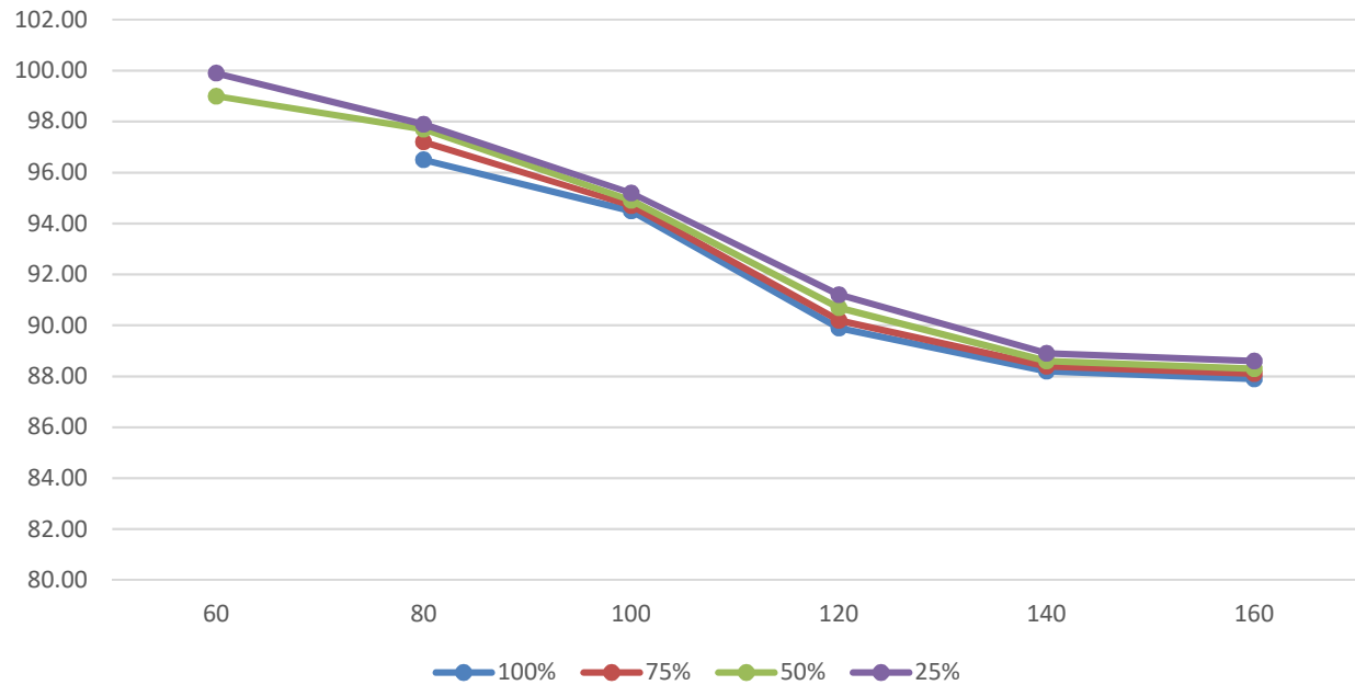
SONIC SC-850 Thermal Efficiencies @ 40°F ΔT
