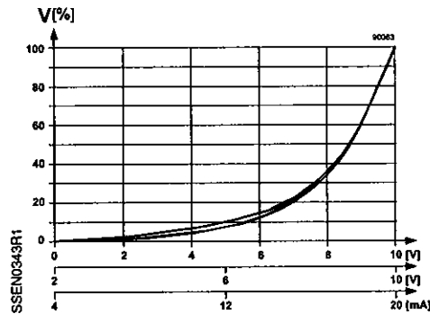
Figure 8. Equal Percentage.
