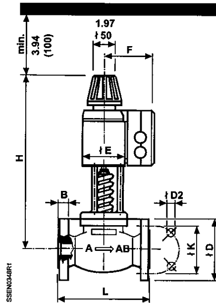
Figure 15. Dimensions in Inches (Millimeters).
