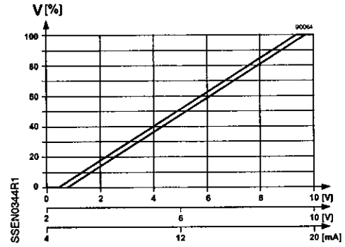
Figure 9. Linear.
