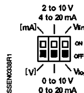
Figure 3. Configuration DIP Switches.
