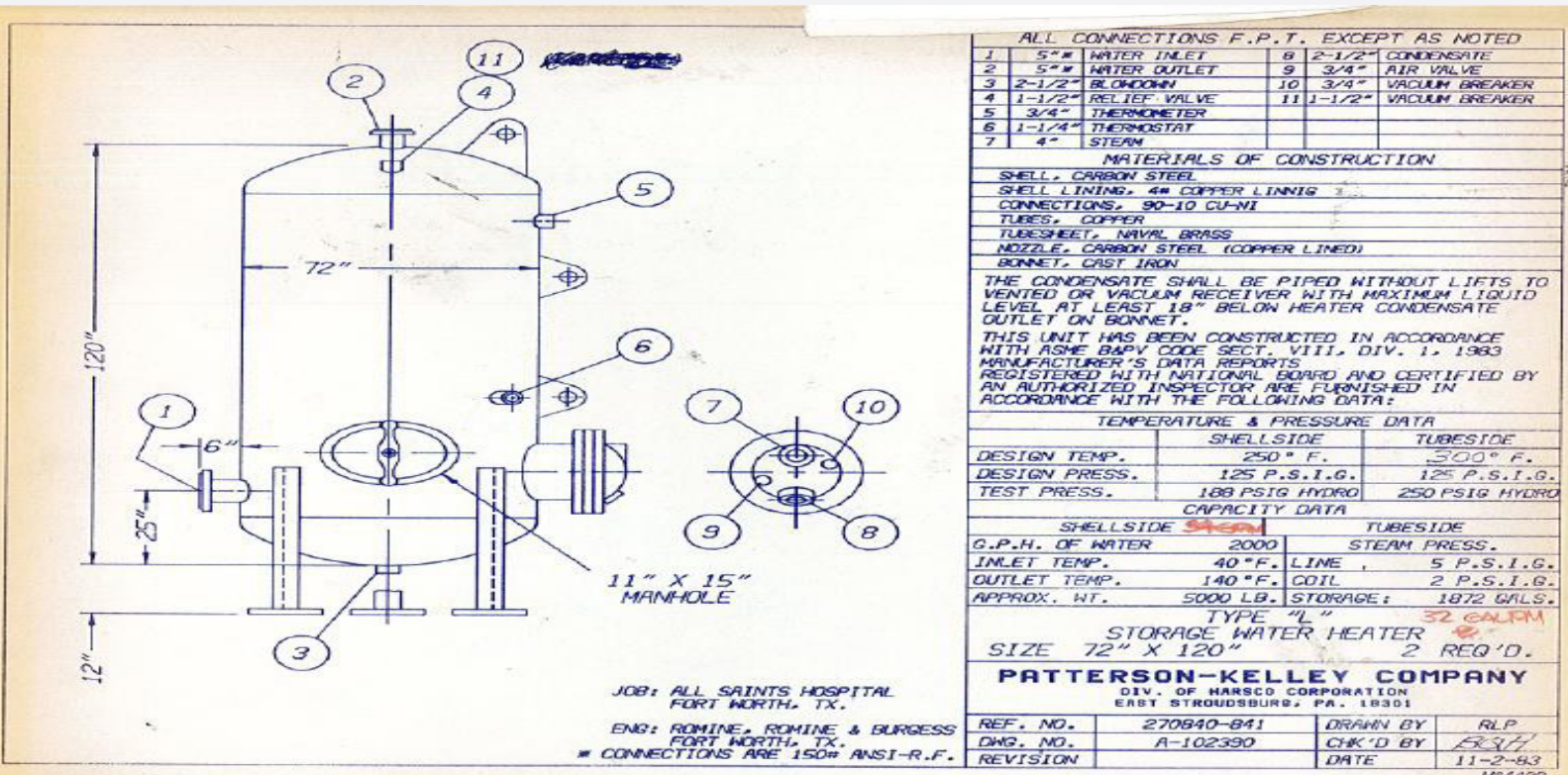
Drawing of Original Storage Water Heater Tank: Model 10-42 Type "L" Storage Water Heater 72" X 120"
